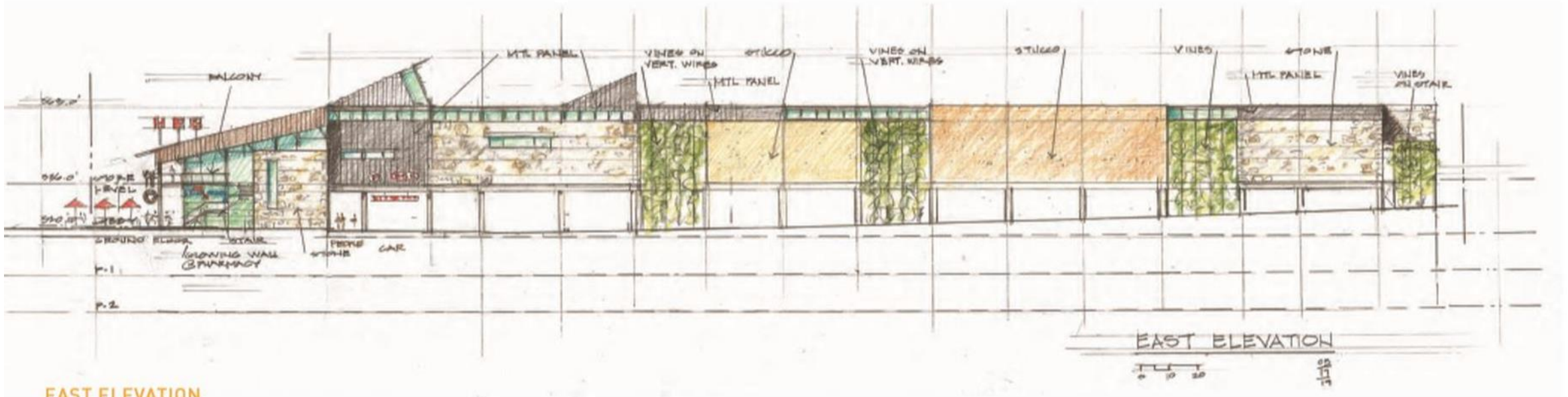
EAST ELEVATION
